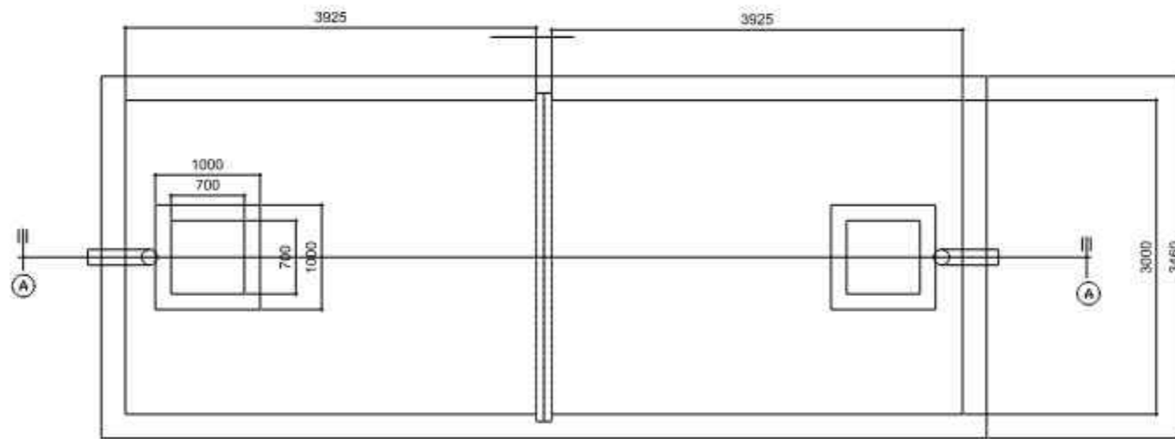
PLAN SCALE 1:40
